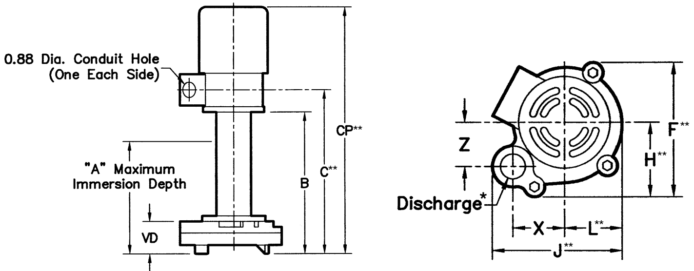
Pump Dimensional & Specification Data
